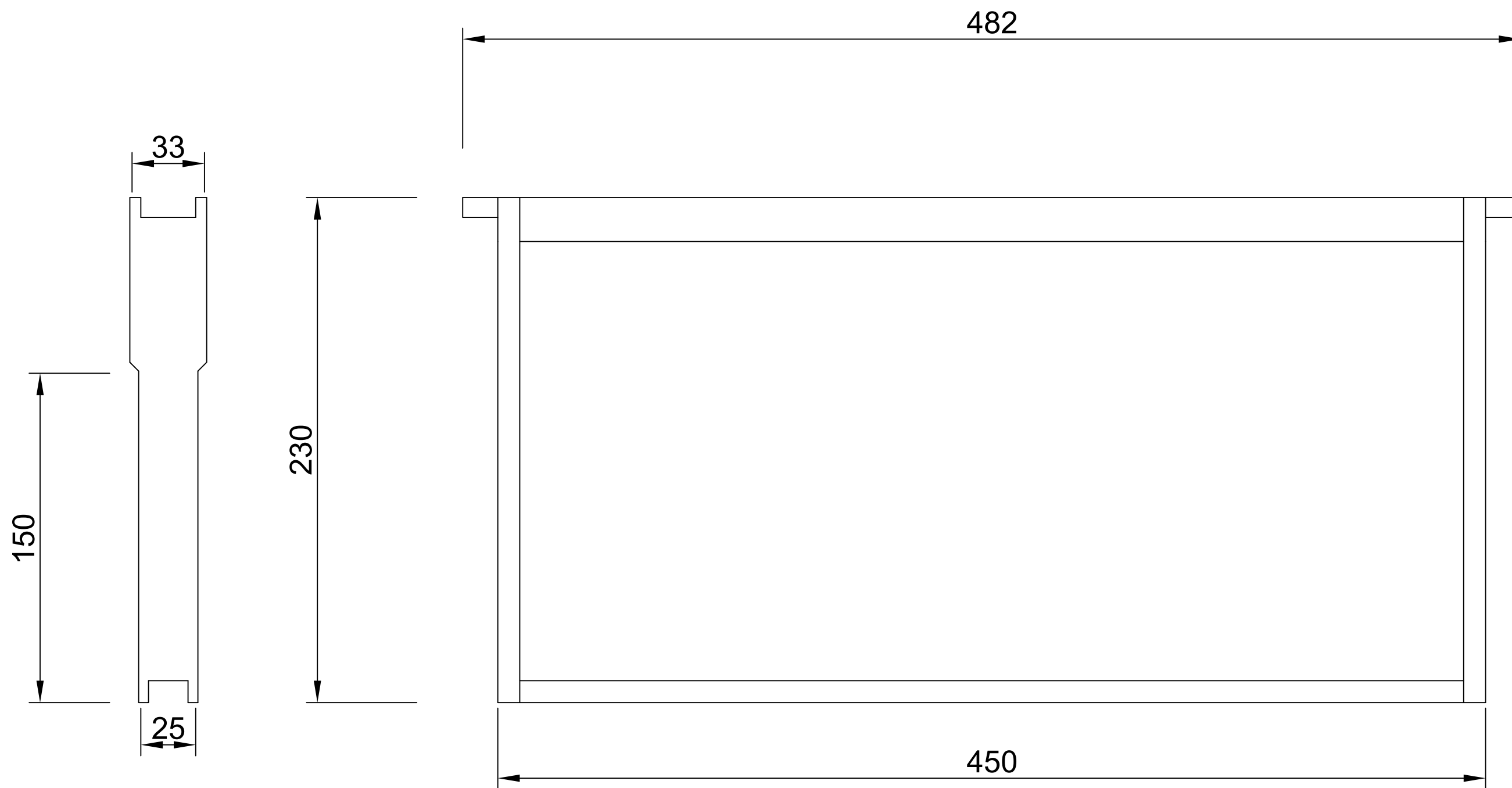
full depth frame elevation: scale 1:2 at a3
